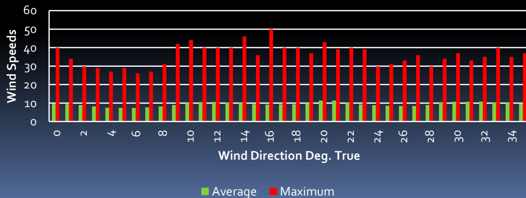
Wind Speeds by Direction Halifax Airport, NS 2000-2019
