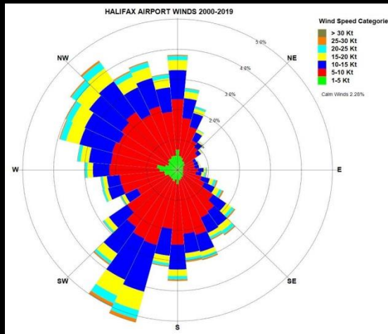
Wind Speeds by Direction Halifax Airport, NS 2000-2019
